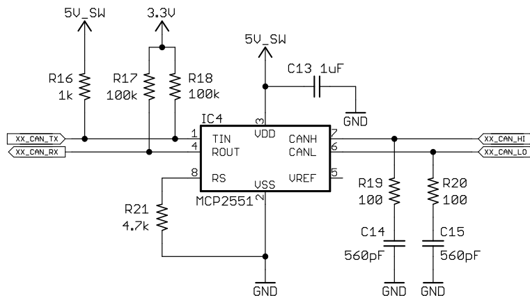
Figure 12 – MCP2551 CAN Transceiver
