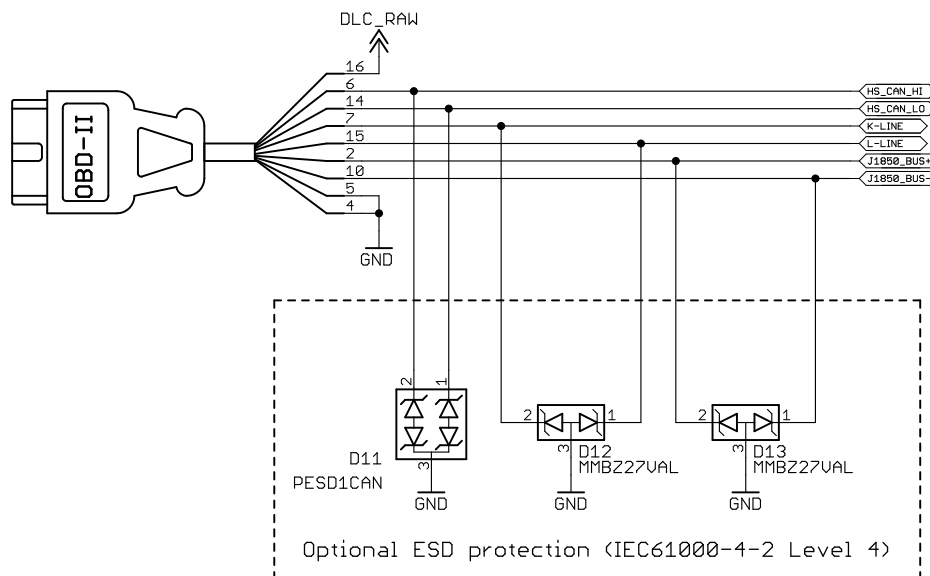
Figure 5 – OBD Port Connector and ESD Protection
