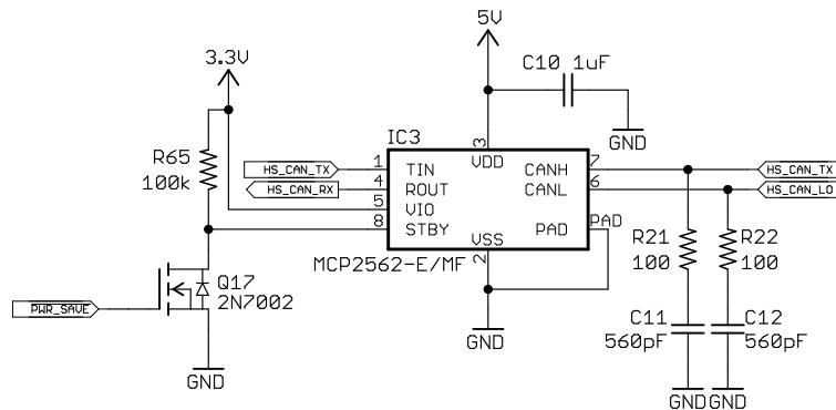
Figure 11 – High Speed CAN Transceiver
