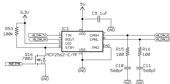
Figure 11 – High Speed CAN Transceiver
