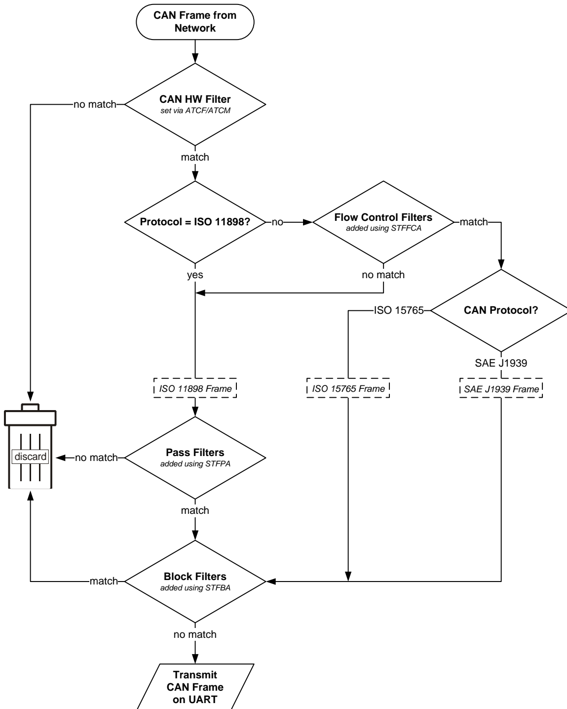
Figure 3 – Message Filtering: CAN Protocols
